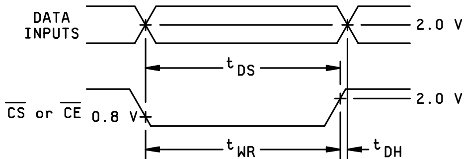
FIGURE 4. Timing diagram.
